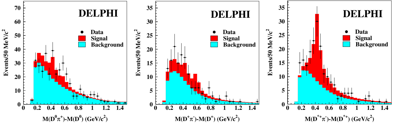
Fig. 6. \Delta_m distributions for right-sign events corresponding to the three D^{(*)}\pi combinations. The fitted signal contributions are superimposed
