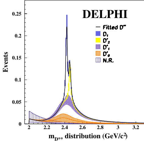
Fig. 7. D^{**} fitted mass distribution. The different components are shown within bands corresponding to the uncertainties of the fitted parameters
