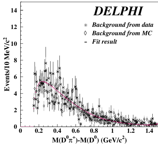
Fig. 5. Comparison between \Delta_m distributions obtained for combinatorial background events selected in the sidebands for real data (stars) and simulation (diamonds) corresponding to the channel D^0\pi^+ in the 1994–1995 data sample. The two distributions have been normalized to the same number of entries. The curve fitted to simulated events has been superimposed
