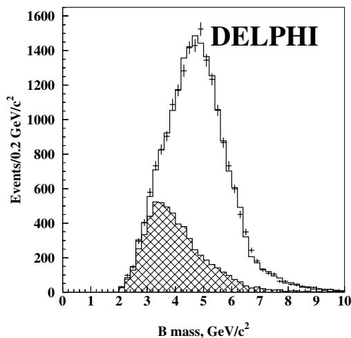
Fig. 11. Reconstructed B mass. Points are the data, histogram is the simulation with the signal clear and the background hatched
