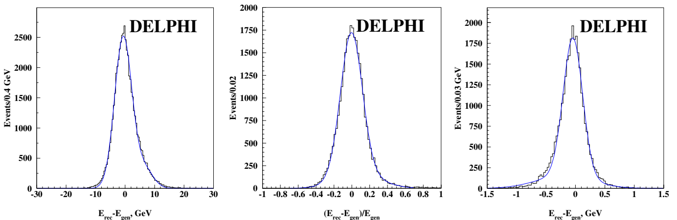
Fig. 9. The resolution on the missing energy (left), the fractional resolution on the reconstructed B hadron energy (centre) and resolution on the E_\ell^* energy (right) estimated with simulation for signal B \rightarrow X_c\ell\bar{\nu}_\ell events
