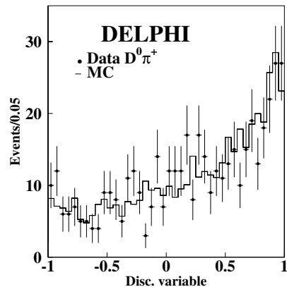
Fig. 4. Discriminant variable distributions for D^{*+} \rightarrow D^0 \pi^+ candidates selected in data (points with error bars) and in simulated hadronic Z decays (histogram)
