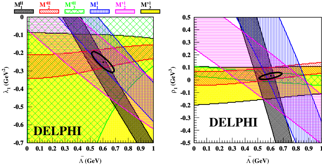
Fig. 15. The projection of the constraints of the six measured moments on the \bar{\Lambda} - \lambda_1 (left) and \bar{\Lambda} - \rho_1 (right) planes. The bands correspond to the total measurement accuracy and are given by keeping all the other parameters at their central values. The ellipses represent the 1\sigma contours and include correlations between the parameters
