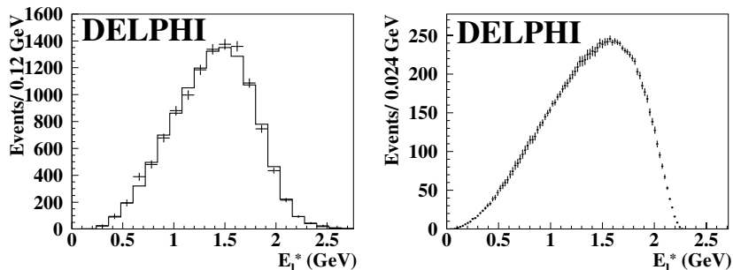
Fig. 12. The resulting E_\ell^* spectrum for samples enriched (left) and depleted (right) in B \rightarrow X_c \ell \bar{\nu}_\ell decays using the separating variable. The data are shown as crosses while the simulation is shown as histograms. The different sources of background, shown shaded, are from bottom to top: b \rightarrow \bar{c} \rightarrow \ell , b \rightarrow c \rightarrow \ell , other lepton sources including decays in flight and converted photons, c \rightarrow \ell , misidentified hadrons. In the lower plots the efficiencies for the selection are shown, as a function of E_\ell^*
