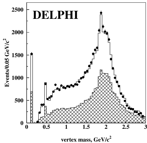
Fig. 8. Mass distribution of the reconstructed charm vertex. The peaks at 0.14 and 0.5 \text{GeV}/c^2 correspond to vertices consisting of a single \pi or K , respectively. Points are the data, while the histogram is the simulation with the signal clear and the background hatched
