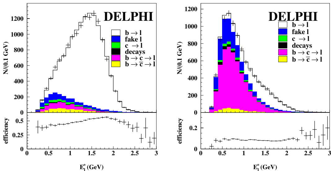
Fig. 12. The resulting E_\ell^* spectrum for samples enriched (left) and depleted (right) in B \rightarrow X_c \ell \bar{\nu}_\ell decays using the separating variable. The data are shown as crosses while the simulation is shown as histograms. The different sources of background, shown shaded, are from bottom to top: b \rightarrow \bar{c} \rightarrow \ell , b \rightarrow c \rightarrow \ell , other lepton sources including decays in flight and converted photons, c \rightarrow \ell , misidentified hadrons. In the lower plots the efficiencies for the selection are shown, as a function of E_\ell^*
