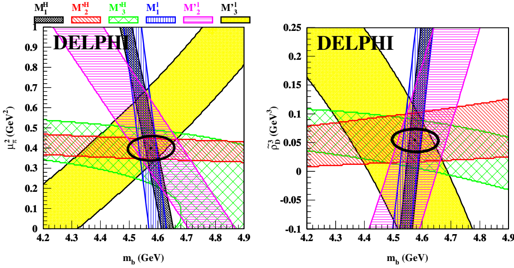
Fig. 14. The projection of the constraints of the six measured moments on the m_b(1 \text{ GeV}) - \mu_\pi^2(1 \text{ GeV}^2) (left) and m_b(1 \text{ GeV}) - \tilde{\rho}_D^3 (right) planes. The bands correspond to the total measurement accuracy and are given by keeping all the other parameters at their central values. The ellipses represent the 1\sigma contours and include correlations between the parameters
